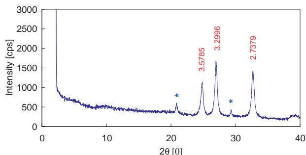
Fig. 4. XRD of the fullerodendron/vaterite composite. The asterisk (*) denotes the diffraction angle caused by calcite, indicating negligible contamination.
