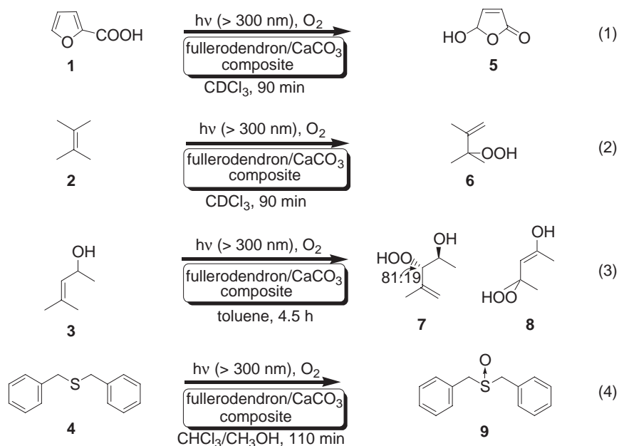
Scheme 1. Photooxygenation reactions carried out with the composite material in heterogeneous condition.
