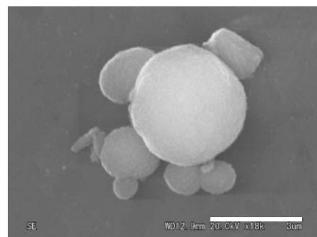
Fig. 5. SEM image of fullerodendron/vaterite composite material (scale bar = 3\text{ }\mu\text{m} ).
