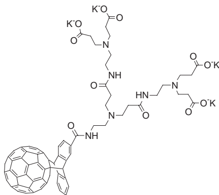
Fig. 2. Structure of fullerodendron ( I ).
