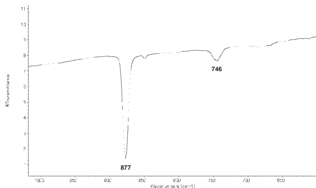
Fig. 3. FT-IR spectrum of \text{CaCO}_3 crystals in the fullerodendron/vaterite composite.
